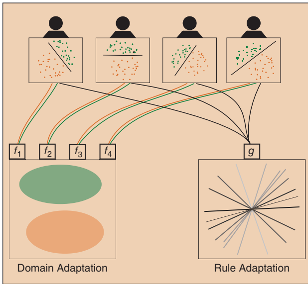
FIGURE 1 Given a set of training datasets (top) there are two ways to model the similarities shared by them. Domain adaptation (left) refers to the strategy of attempting to find a transformation to a data space in which a single decision rule will classify all samples. Instead of learning a new rule for the new data, data is simply transformed to the invariant space. Rule adaptation (right) is the strategy of attempting to learn the structure of the classification rules. New datasets are faced with a much smaller search space of possible rules which allows for much faster learning of novel decision boundaries.
