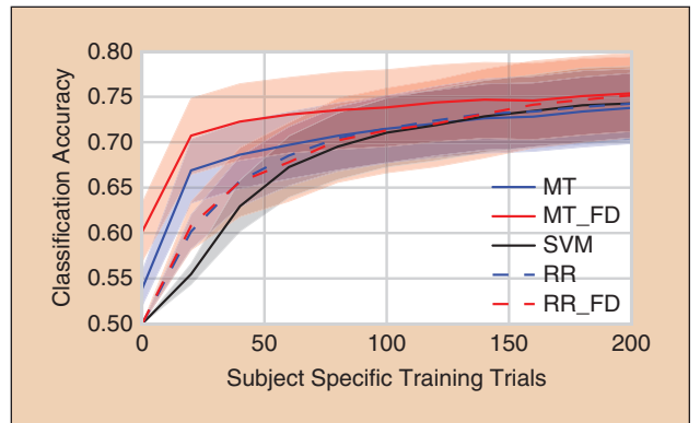
FIGURE 3 Mean and STD (shaded) for classification accuracy of MT and single-subject conditions across the ten subjects. Classification values for the multitask algorithms are identical to those shown in Figure 2. The control algorithms were trained on data exclusively from the test subject, and are compared against classification using Algorithm 1 (MT, solid blue) and Algorithm 3 (MT_FD, solid red). Displayed control algorithms are ridge regression using the standard regression method (RR, dashed blue), ridge regression using the FD regression method (RR_FD, dashed red) and SVM (SVM, solid black). The multitask algorithm with FD regression estimation performs better on average regardless of the number of trials, though single-subject ridge regression with the FD regression method manages to equal its performance at 200 training trials.
