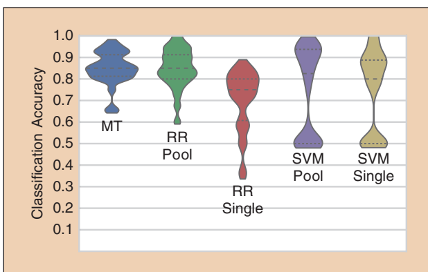
FIGURE 5 Density plot of classification accuracy over sessions for each algorithm. MT corresponds to multitask learning using Algorithm 2 and RR corresponds to ridge regression using the FD regression method. Dashed line corresponds to median for the distribution and dotted lines show upper and lower quartiles. Classification accuracies using the pooled FD regression and multitask learning have a higher minimum classification accuracy than any other method.
