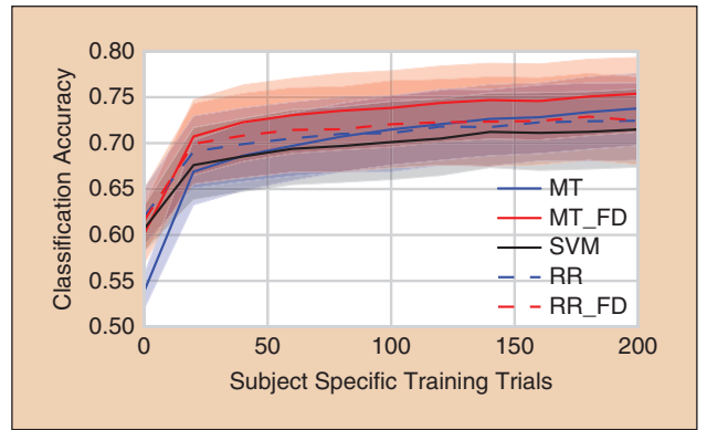
FIGURE 2 Mean and STD (shaded) for classification accuracy of MT and pooled conditions across the ten subjects. The control algorithms were trained on data pooled across training subjects, and are compared against classification using Algorithm 1 (MT, solid blue) and Algorithm 3 (MT_FD, solid red). Displayed control algorithms are ridge regression using the standard regression method (RR, dashed blue), ridge regression using the FD regression method (RR_FD, dashed red) and SVM (SVM, solid black). The FD formulation of the multitask learning has comparable performance with few training trials to pooled regression and both multitask algorithms manage to improve more than the pooled controls given a larger number of training trials.
